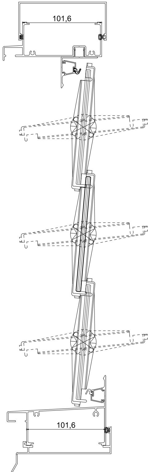
HEAD & SILL
