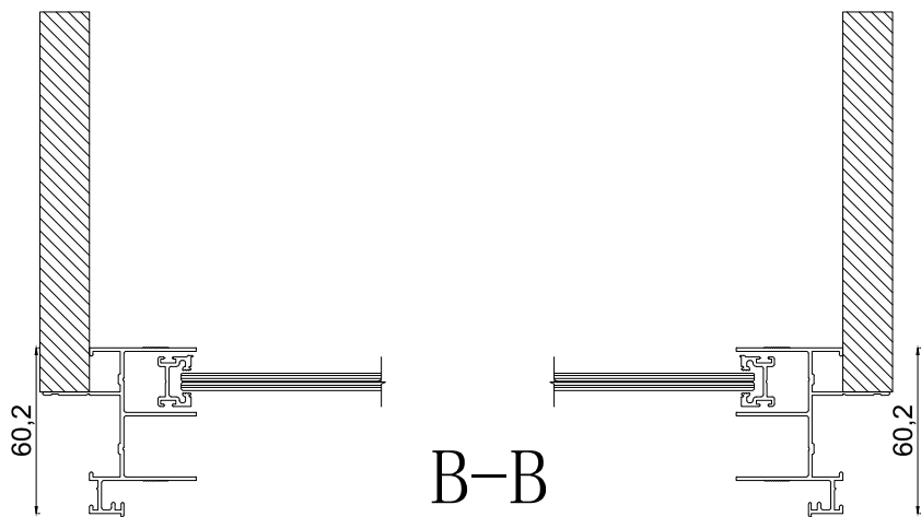
DOUBLE HUNG WINDOW
