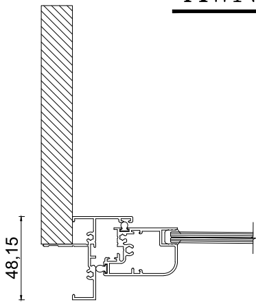
AWNING WINDOW
