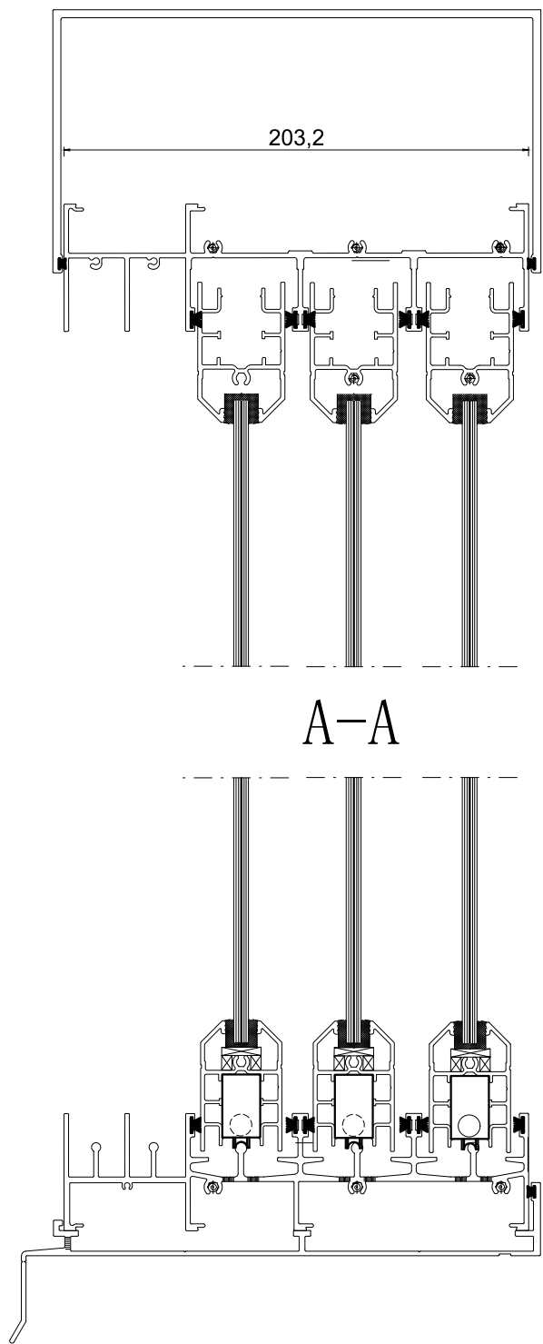
HEAD & SILL
