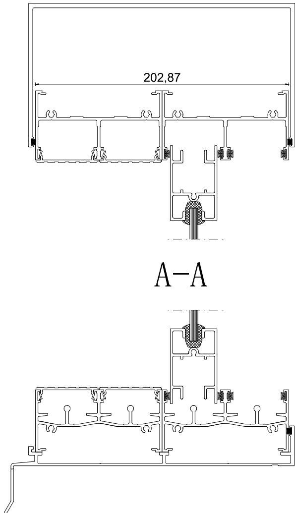
HEAD & SILL
