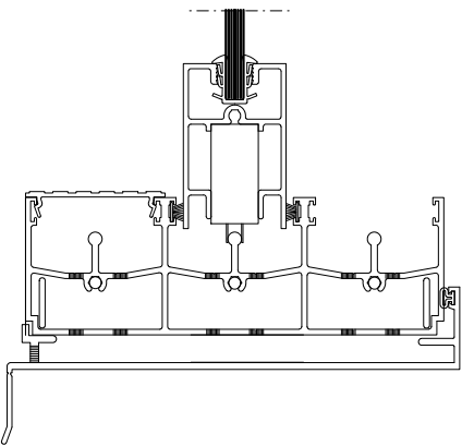
HEAD & SILL
