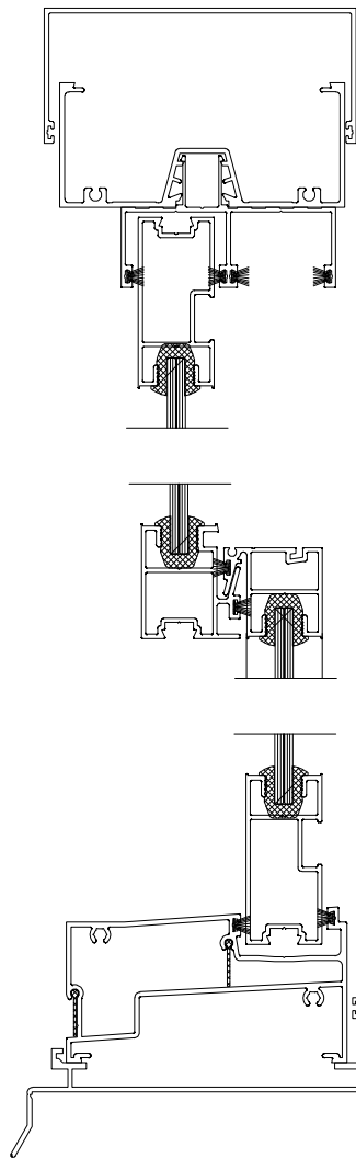
HEAD & SILL
