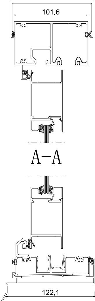
HEAD & SILL
