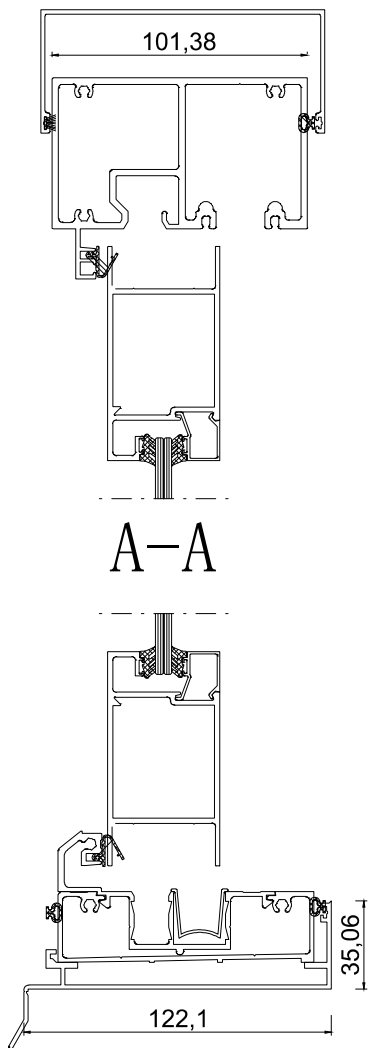
HEAD & SILL
